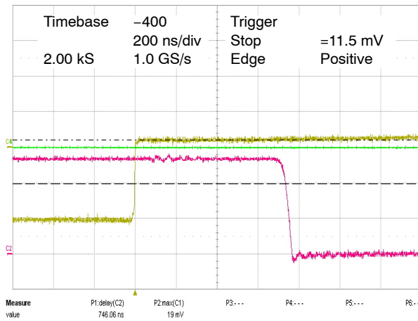
Figure 10. 10 mV Overdrive
