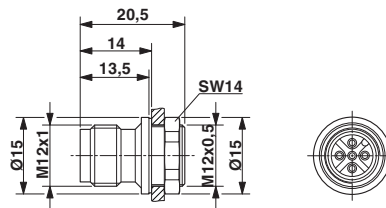
Dimensioned drawing
