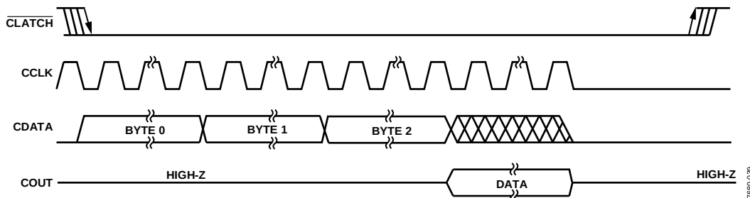
Figure 56. SPI Read from ADAU1761 Clocking (Single-Word Read Mode)
