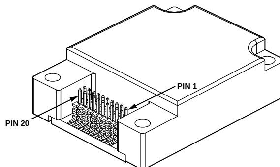
Figure 6. Pin Locations
