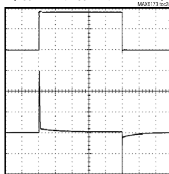
LOAD TRANSIENT ( V_{OUT} = 10V , C_{OUT} = 0 , 0 TO 20mA)
