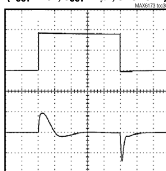
LOAD TRANSIENT ( V_{OUT} = 10V , C_{OUT} = 1\mu F , 0 TO 20mA)
