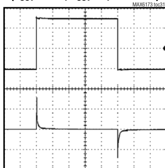
LOAD TRANSIENT ( V_{OUT} = 2.5V , C_{OUT} = 0 , 0 TO -2mA)
