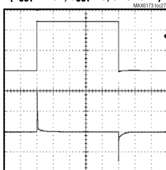
LOAD TRANSIENT ( V_{OUT} = 2.5V , C_{OUT} = 0 , 0 TO 20mA)
