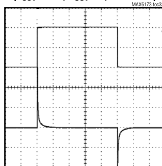
LOAD TRANSIENT ( V_{OUT} = 10V , C_{OUT} = 0 , 0 TO -2mA)
