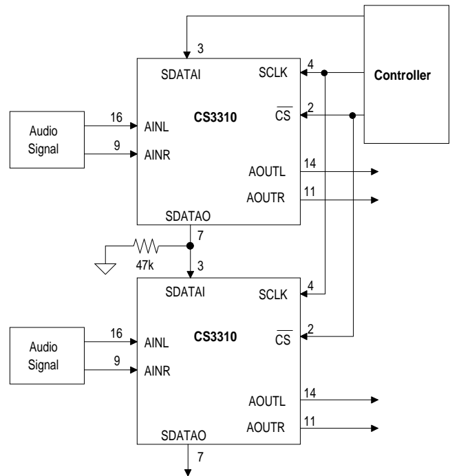
Figure 4. Daisy Chaining Diagram
