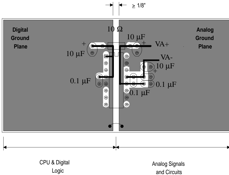
Figure 6. Recommended 2-Layer PCB Layout
