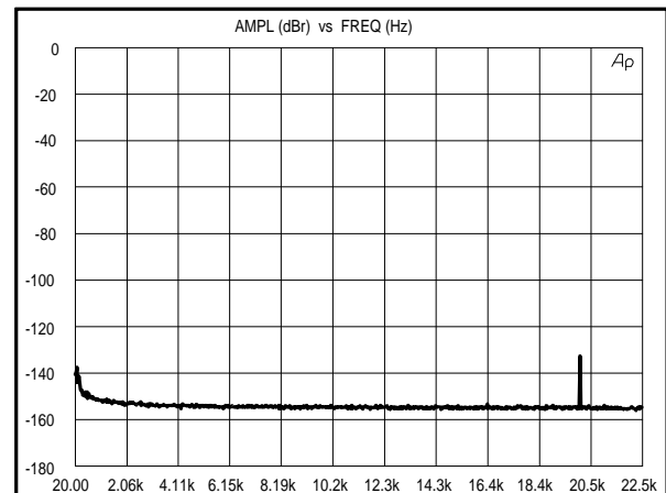
Figure 10. 20 kHz Crosstalk
