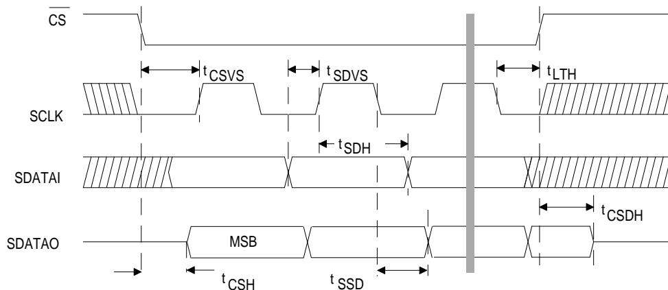
Figure 1. Serial Port Timing Diagram
