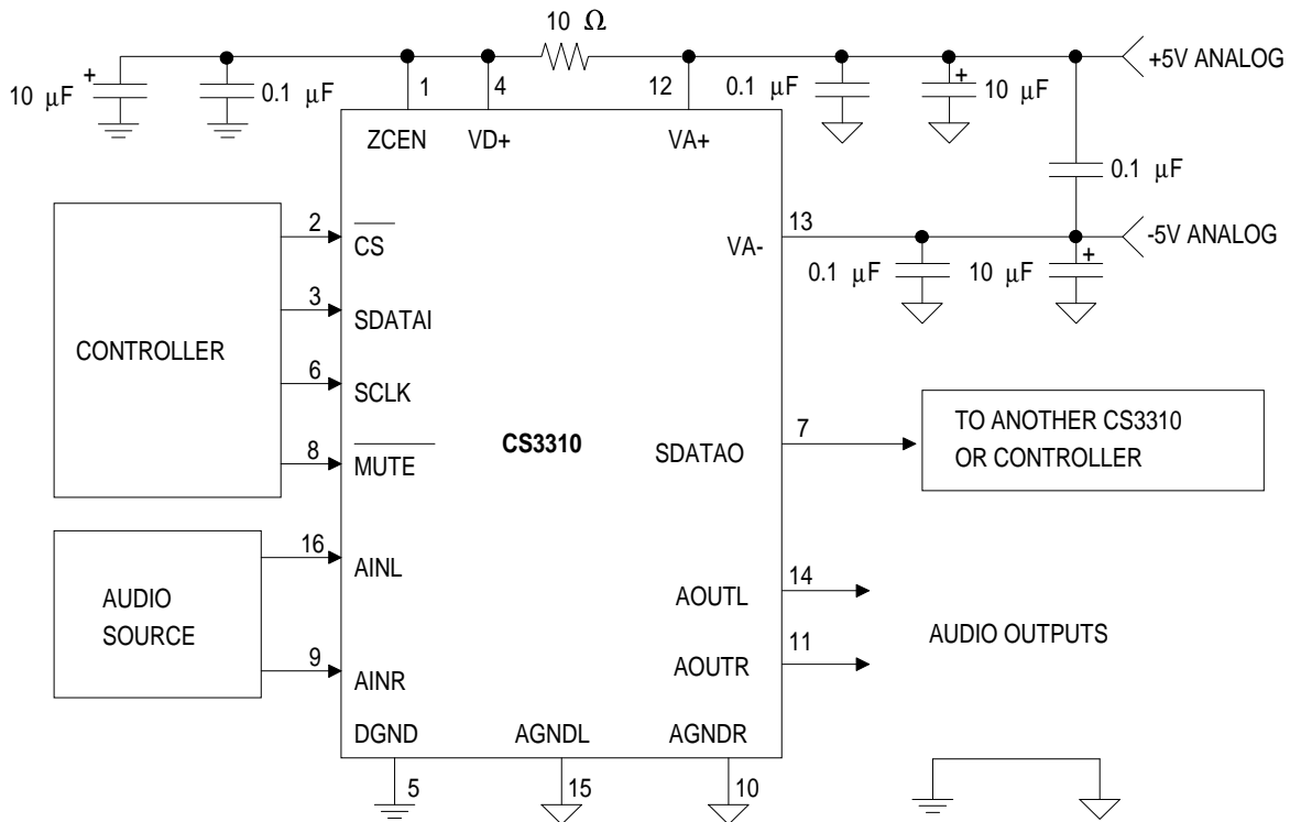
Figure 2. Recommended Connection Diagram
