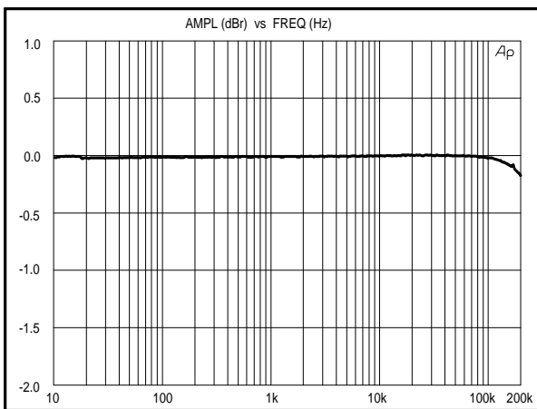
Figure 8. Frequency Response -20 dB Input
