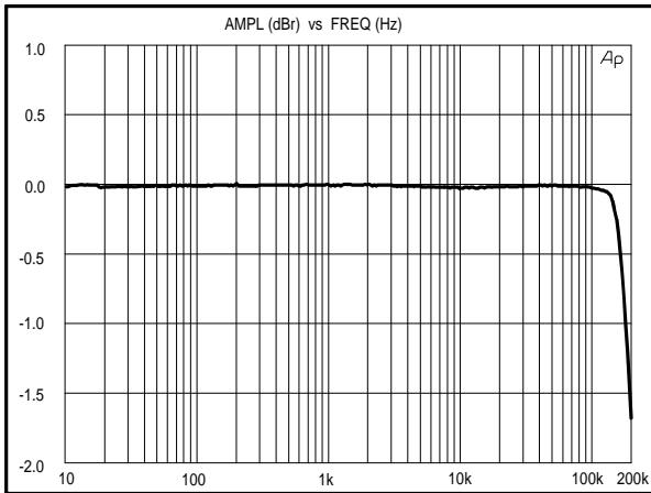
Figure 7. Frequency Response Full scale Input
