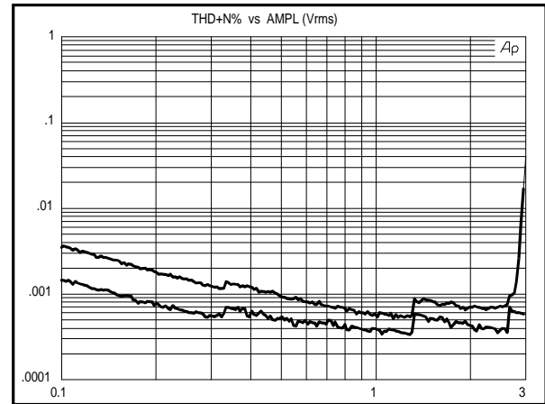
Figure 9. THD+N vs AMP
