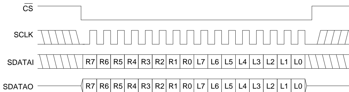
L0 = Left Channel Least Significant Bit R0 = Right Channel Least Significant Bit L7 = Left Channel Most Significant Bit R7 = Right Channel Most Significant Bit SDATAI is latched internally on the rising edge of SCLK SDATAO transitions after the falling edge of SCLK SDATAO bits reflect the data previously loaded into the CS3310
