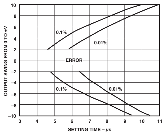
Figure 14. Output Swing and Error vs. Settling Time
