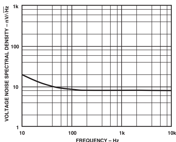
AD795 Voltage Noise Spectral Density
