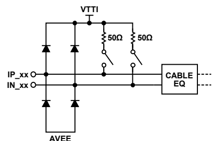
Figure 19. High Speed Input Simplified Schematic
