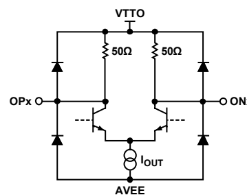
Figure 20. High Speed Output Simplified Schematic
