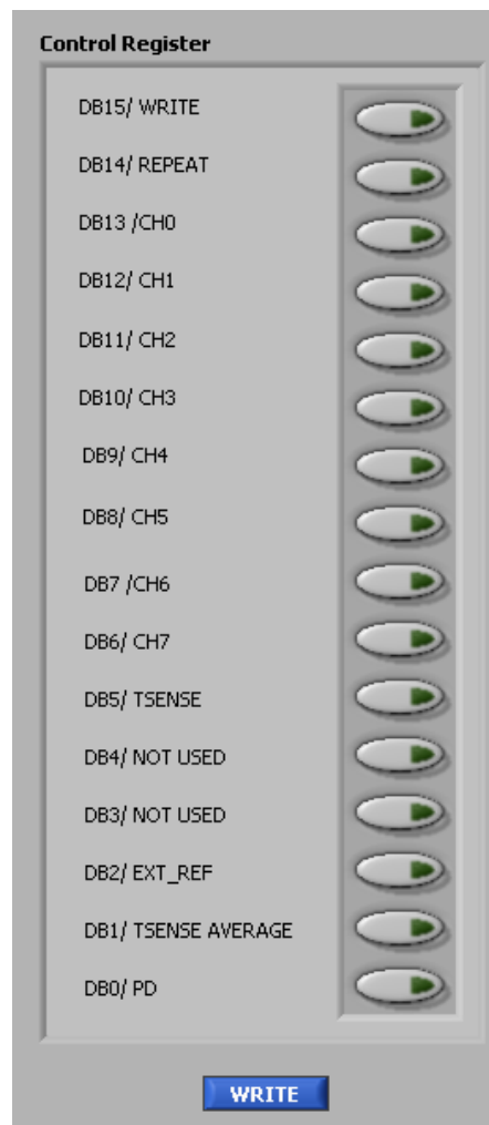
Figure 4. Control Register
