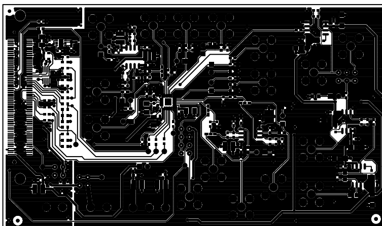
Figure 11. Component Side Silkscreen
