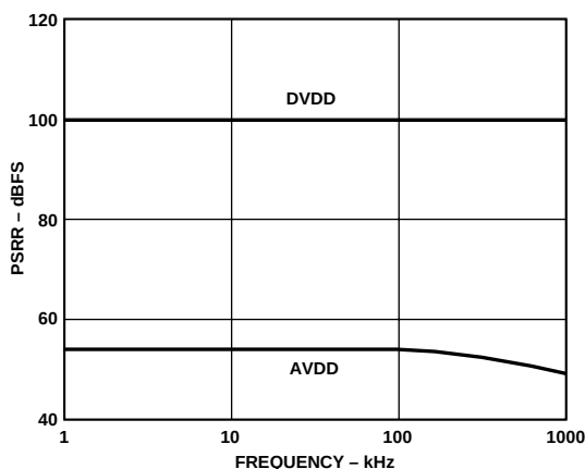
Figure 45. AD9243 PSSR vs. Frequency
