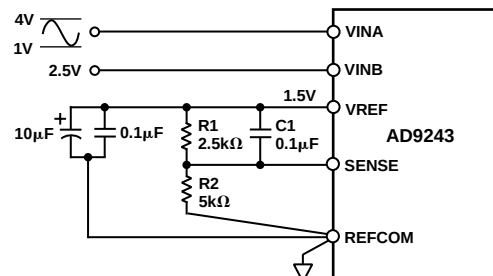
Figure 38. Resistor Programmable Reference (3 V p-p Input Span, V_{CM} = 2.5 V)
