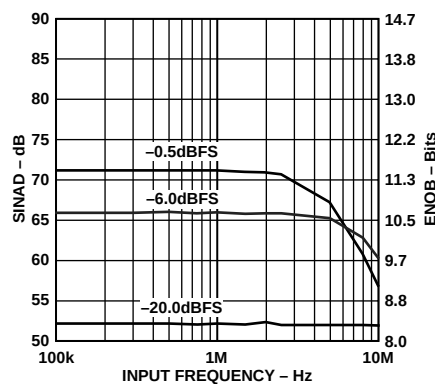
Figure 14. SINAD vs. Input Frequency (Input Span = 2 V, V_{CM} = 2.5\text{ V} )
