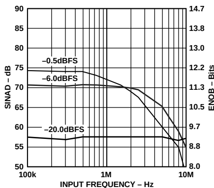
Figure 17. SINAD vs. Input Frequency (Input Span = 5 V, V_{CM} = 2.5\text{ V} )
