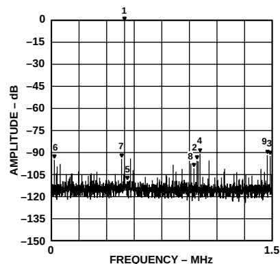
Figure 4. Typical FFT, f_{IN} = 500\text{ kHz} (Input Span = 5 V, V_{CM} = 2.5\text{ V} )
