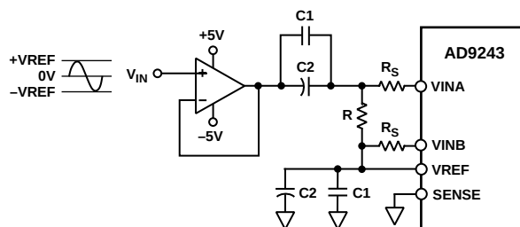
Figure 34. AC-Coupled Input
