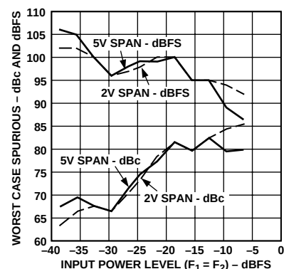
Figure 10. Dual Tone SFDR ( f_1 = 0.95\text{ MHz} , f_2 = 1.04\text{ MHz} , V_{CM} = 2.5\text{ V} )
