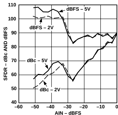
Figure 9. Single Tone SFDR ( f_{IN} = 1.5\text{ MHz} , V_{CM} = 2.5\text{ V} )
