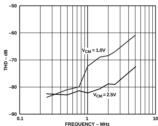
Figure 24. AD9243 THD vs. Frequency for V_{CM} = 2.5 V and 1.0 V ( A_{IN} = -0.5 dB, Input Span = 2.0 V p-p)
