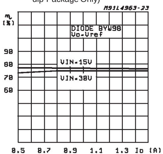
Figure 19: Efficiency vs. Output Current (Powerdip Package Only)
