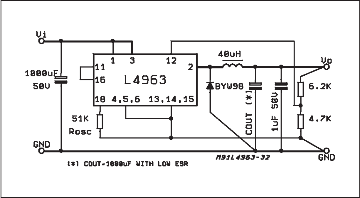
Figure 31: A Minimal Components count for U_o = 12V
