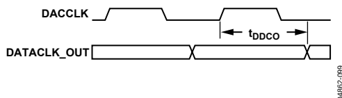
Figure 101. DACCLK to DATACLK_OUT Delay
