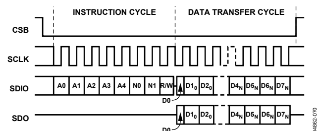
Figure 72. Serial Register Interface Timing, LSB-First Read
