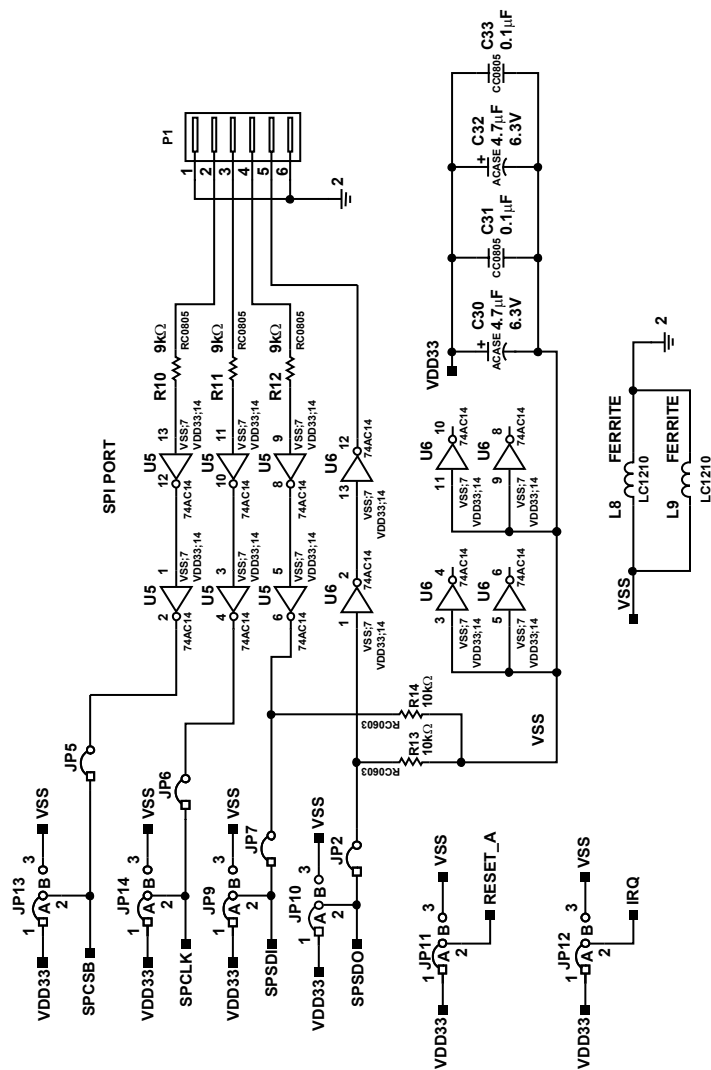
Figure 108. SPI Port Interface, AD973x Evaluation Board, Rev. F
