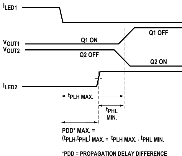
Figure 22. Minimum LED Skew for Zero Dead Time.
