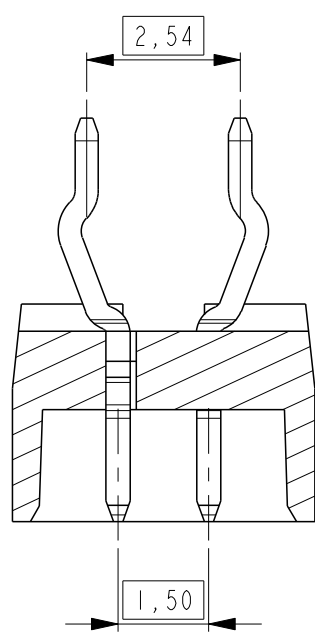
SECTION B-B
