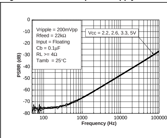
Figure 13. PSRR vs. power supply
