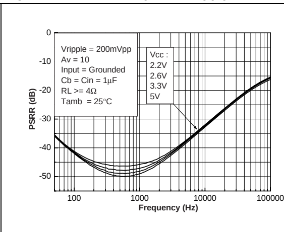
Figure 9. PSRR vs. power supply
