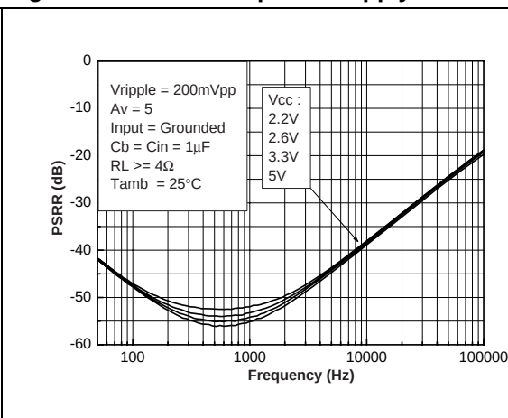
Figure 11. PSRR vs. power supply
