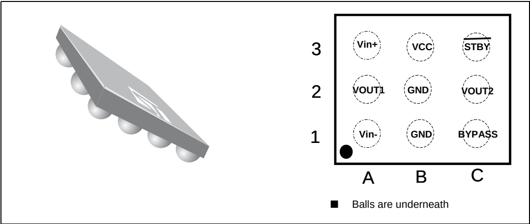
Figure 65. Flip-chip silhouette and pinout (top view)
