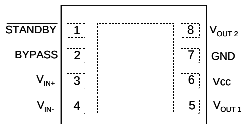
TS4990IQT - DFN8
