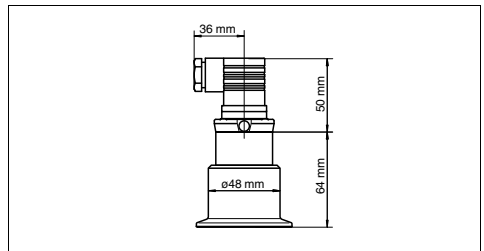
Fig. 16: Version: Process fitting „2“, electrical connection „V“
