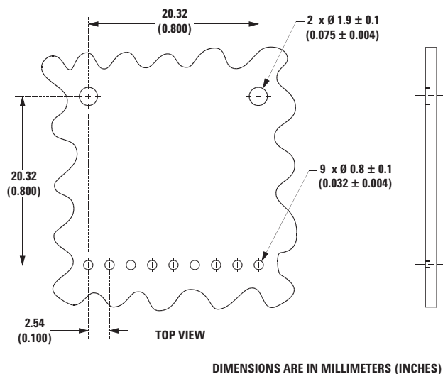
Figure 8. Recommended Board Layout Hole Pattern
