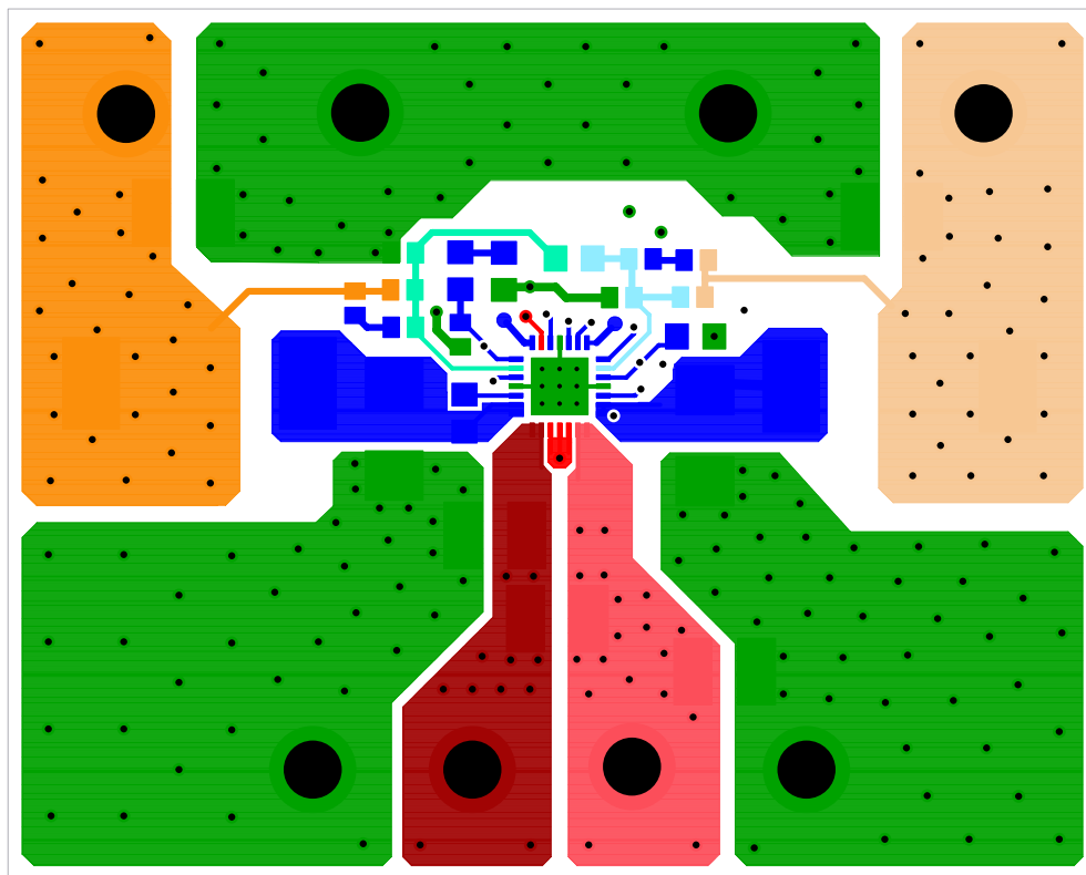
FIGURE 5. TOP LAYER COMPONENT SIDE
