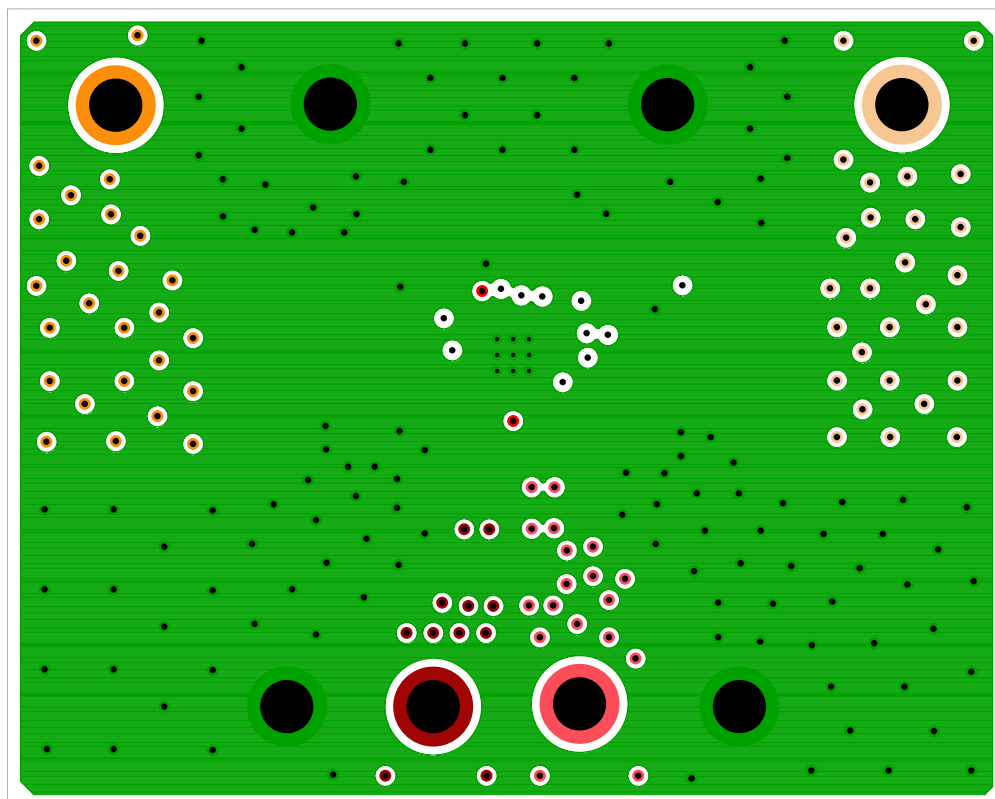
FIGURE 6. LAYER 2
