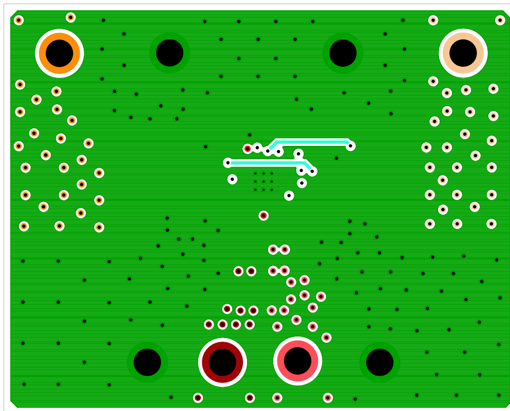
FIGURE 7. LAYER 3
