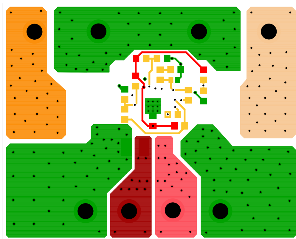
FIGURE 8. BOTTOM LAYER SOLDER SIDE
