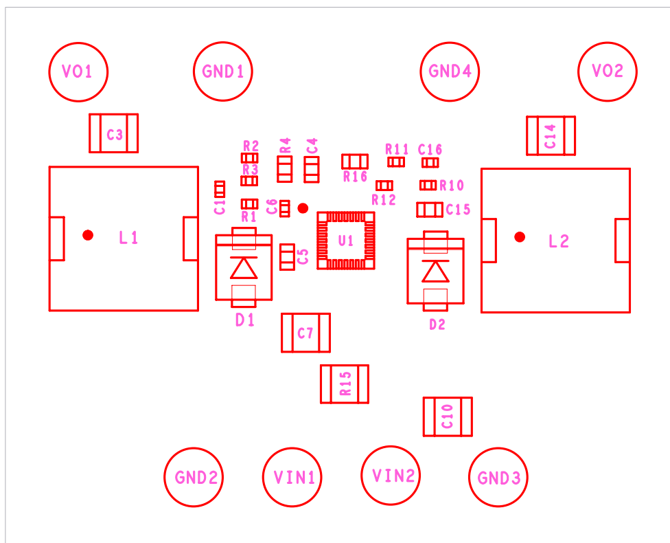
FIGURE 3. TOP ASSEMBLY
