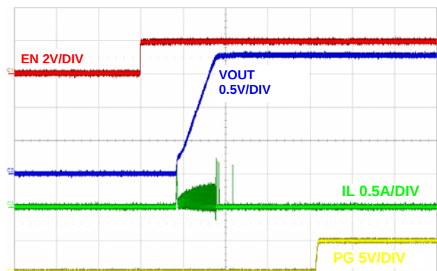
FIGURE 23. SOFT-START AT NO LOAD (PFM), (500µs/DIV)
