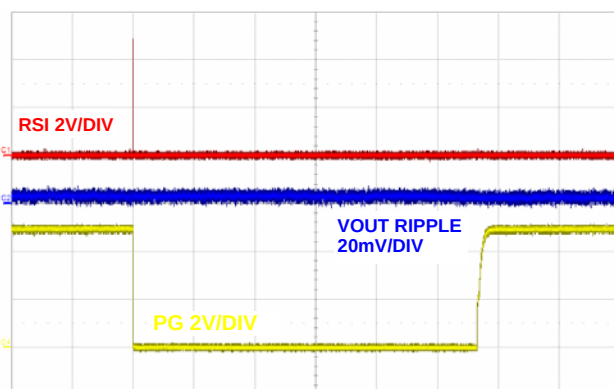
FIGURE 28. RSI RESET (ZOOM OUT), (200µs/DIV)
