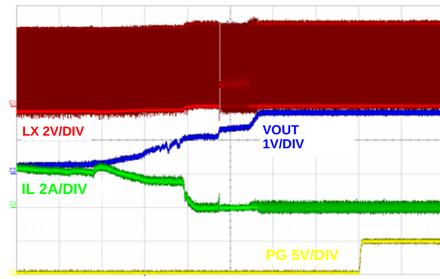
FIGURE 30. OUTPUT SHORT CIRCUIT RECOVERY, (500µs/DIV)
