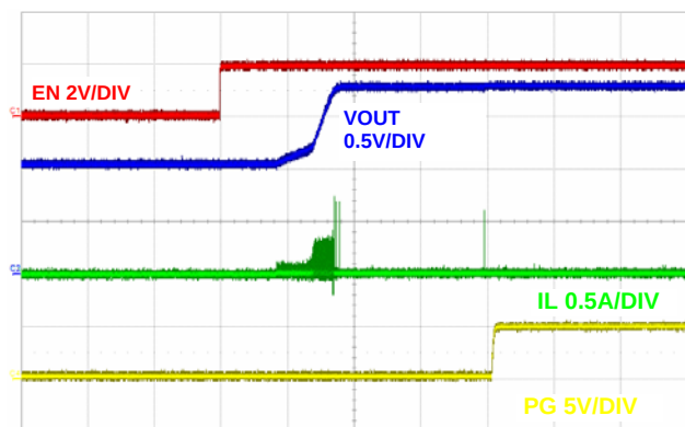
FIGURE 24. SOFT-START WITH PRE-BIASED 1V, (500µs/DIV)
