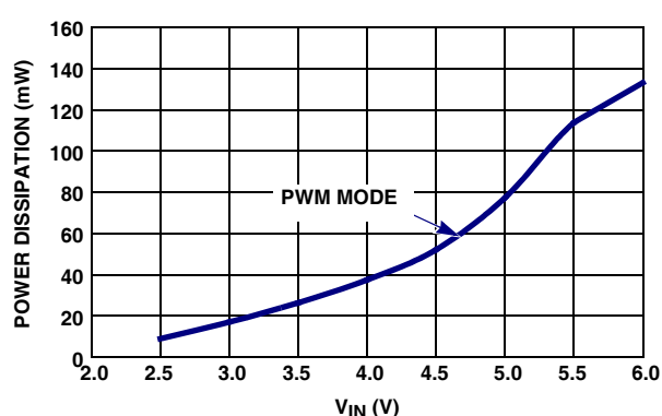
FIGURE 8. POWER DISSIPATION WITH NO LOAD vs V_{IN} (PWM V_{OUT} = 1.8\text{V} )
