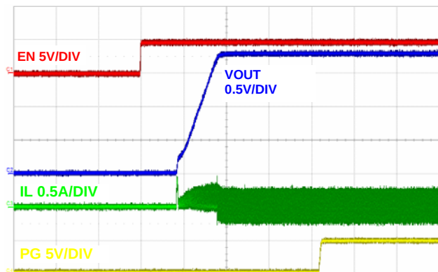
FIGURE 22. SOFT-START WITH NO LOAD (PWM), (500µs/DIV)
