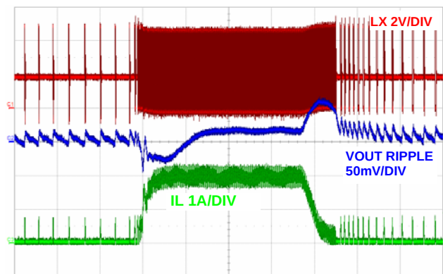
FIGURE 21. LOAD TRANSIENT (PFM), (500µs/DIV)
