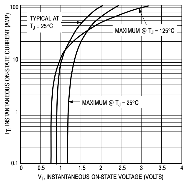
Figure 7. On-State Characteristics
