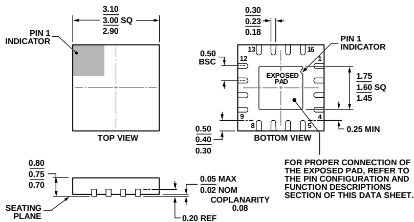
Figure 62. 16-Lead Lead Frame Chip Scale Package [LFCSP_WQ] 3 mm x 3 mm Body, Very Thin Quad (CP-16-22) Dimensions shown in millimeters
