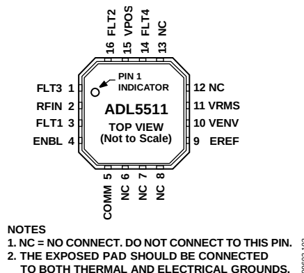
Figure 3. Pin Configuration
