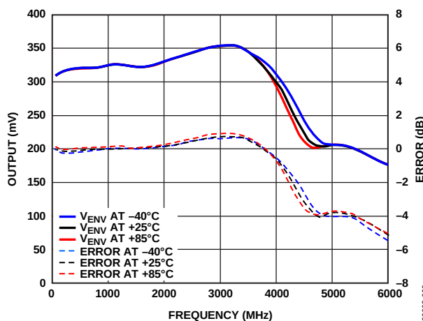
Figure 58. V_{ENV} Output vs. Frequency for a Fixed Input Power, P_{IN} = 0 dBm, Calibration at 1.9 GHz, 25°C
