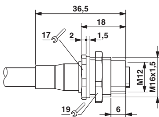
Dimensioned drawing
