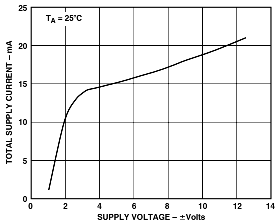
TPC 4. Total Supply Current vs. Supply Voltage
