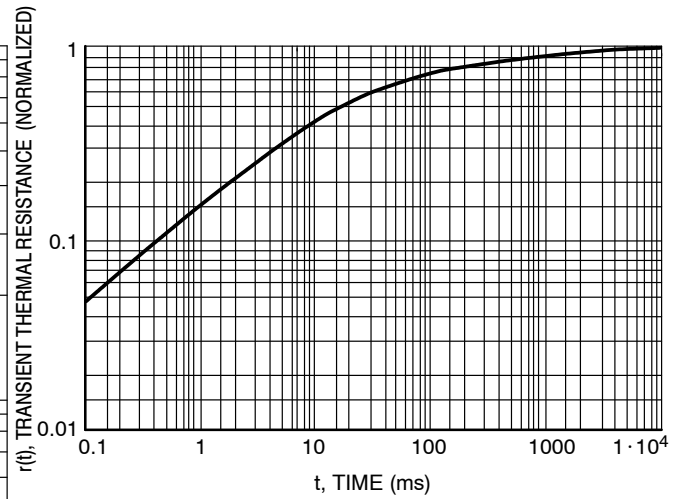
Figure 4. Thermal Response
