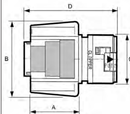
Plug
