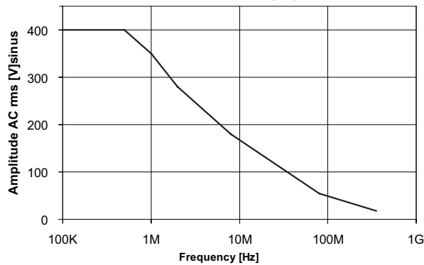
Typical voltage derating PMTG321A (switched to 10:1) Measurement category I
