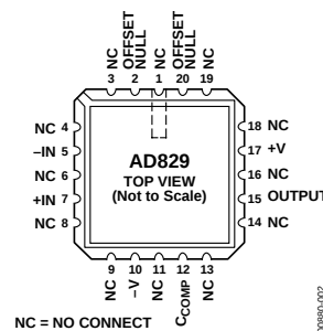
Figure 2. 20-Terminal LCC
