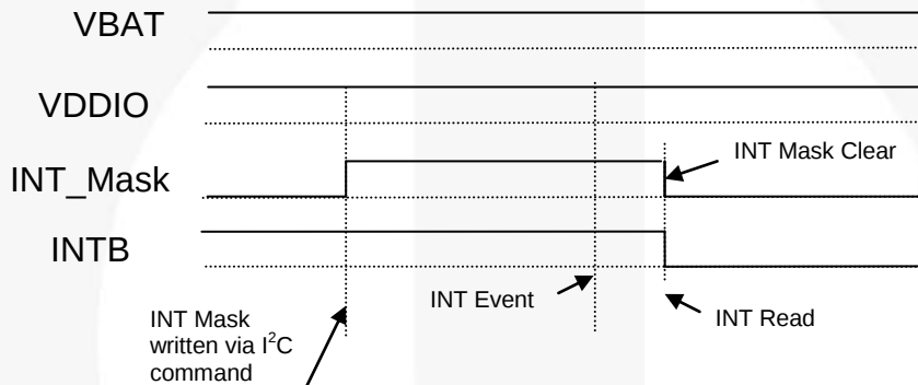
Figure 8. INT Mask to INTB Interrupt Timing Diagram
