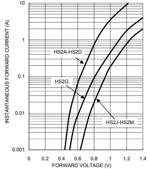
FIG. 5- TYPICAL INSTANTANEOUS FORWARD CHARACTERISRICS
