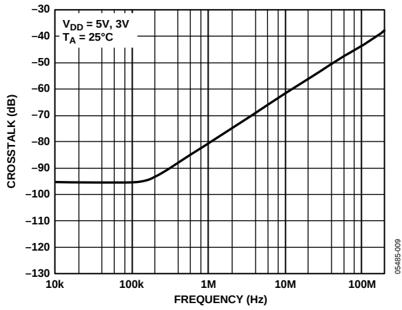
Figure 9. Crosstalk vs. Frequency
