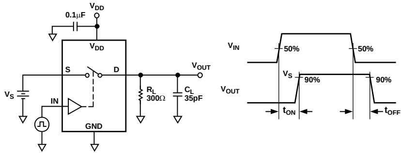
Figure 13. Switching Times
