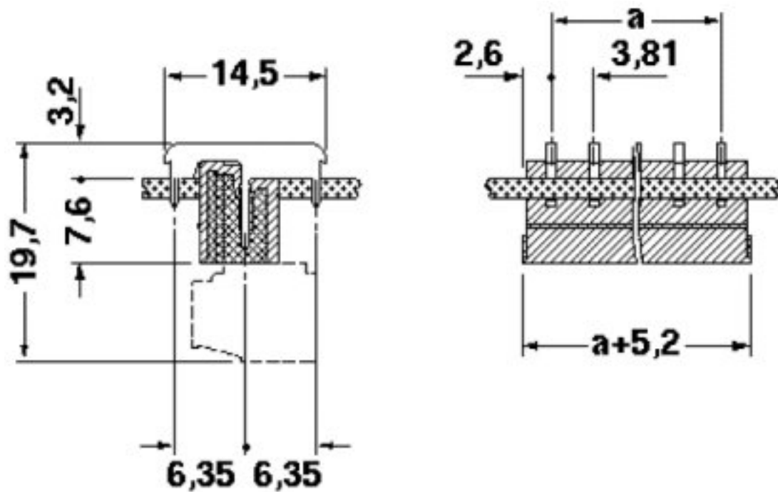
Dimensioned drawing
