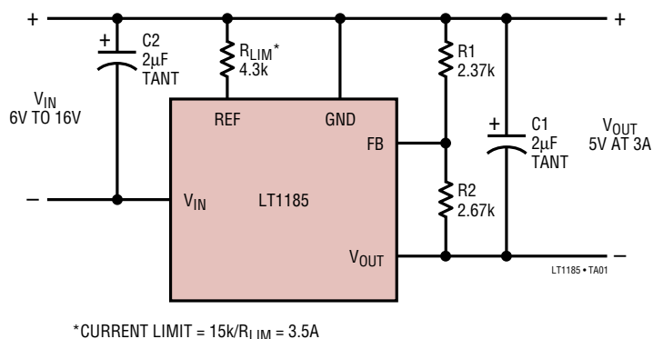
5V, 3A Regulator with 3.5A Current Limit
