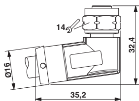
Dimensioned drawing
