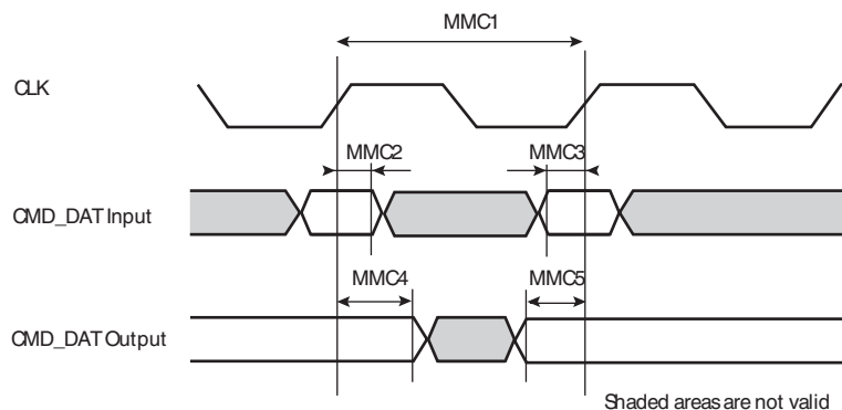
Figure 44-17. MMC Timings
