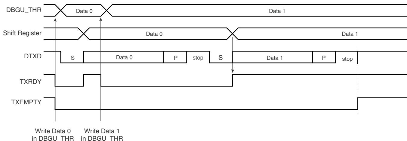
Figure 30-11. Transmitter Control
