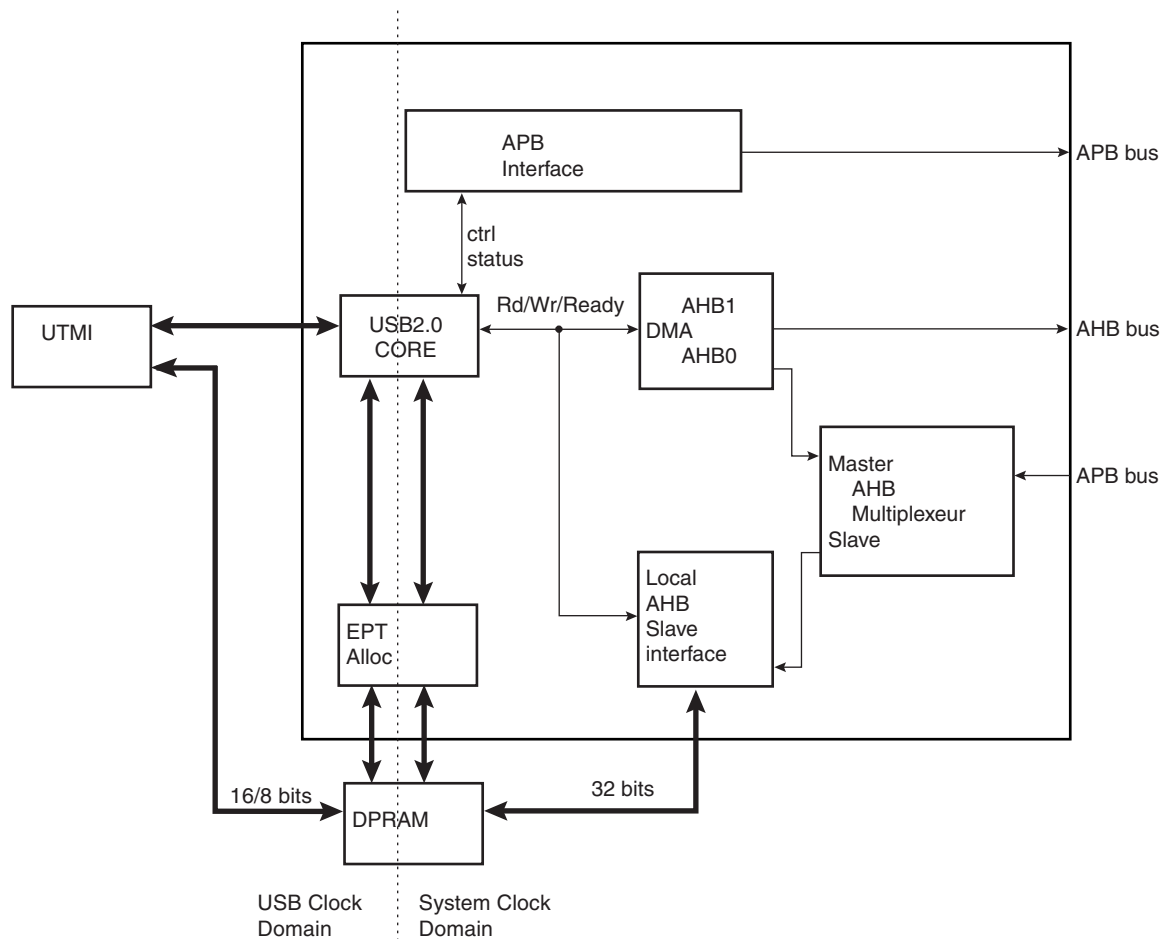
Figure 41-1. Block Diagram:
