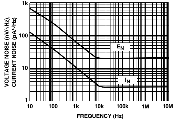
FIGURE 10. VOLTAGE AND CURRENT NOISE vs FREQUENCY
