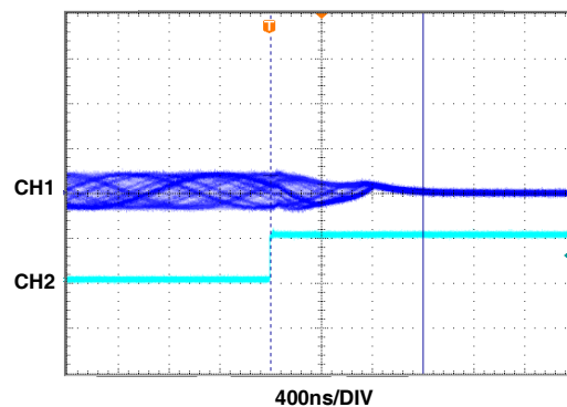
FIGURE 20. ENABLED RESPONSE
