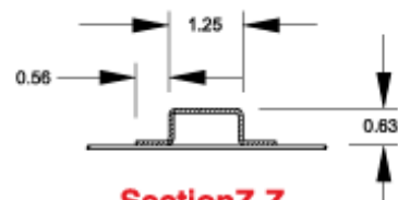
Section Z-Z
