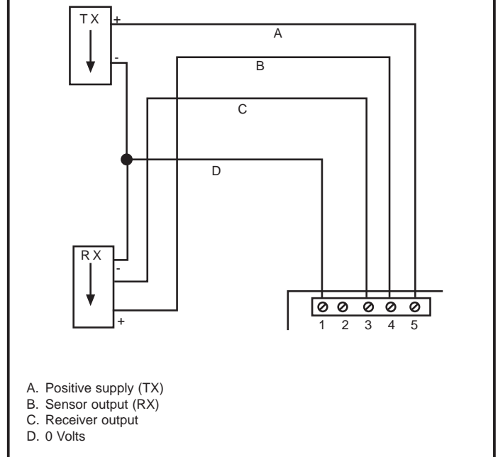
Figure 6 Optical sensors
