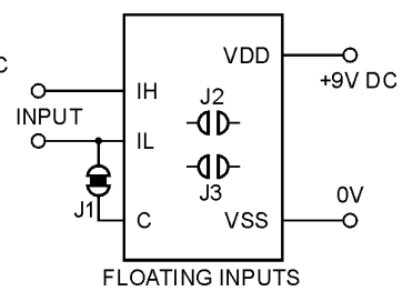
FLOATING INPUTS
