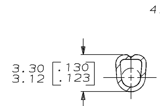
SECTION B-B SCALE 5:1 PRE-CRIMPED
