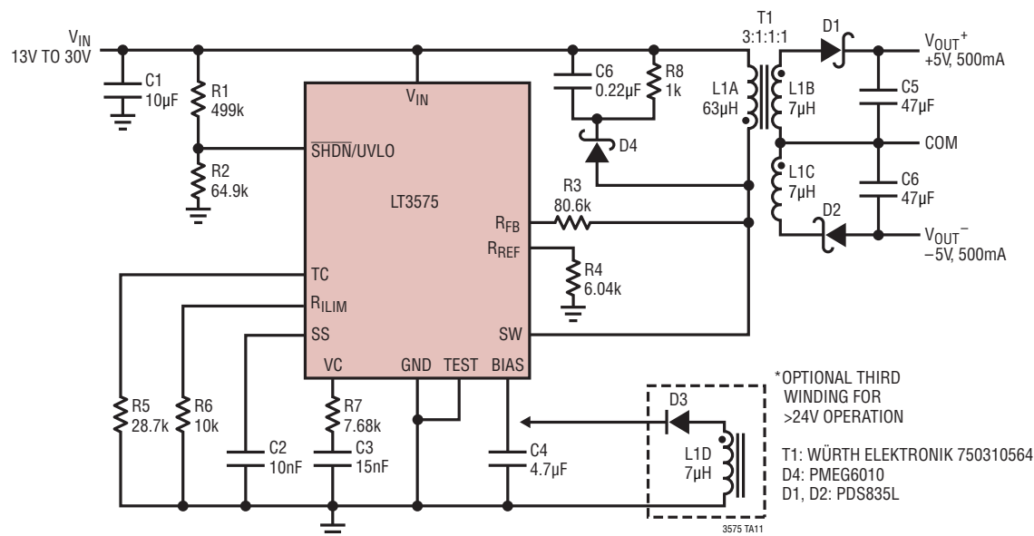
13V to 30V IN , +5V/−5V OUT Isolated Flyback Converter
