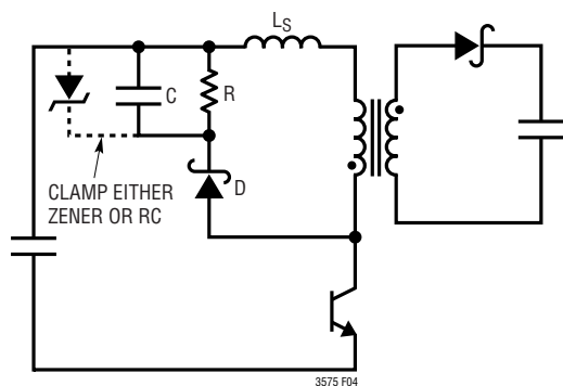
Figure 4. Snubber Clamping
