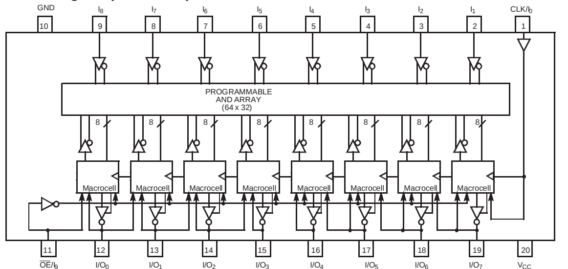
Logic Block Diagram (PDIP/CDIP)
