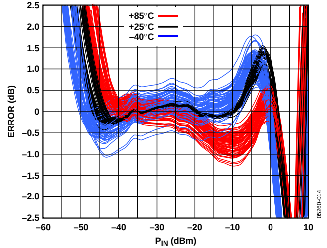
Figure 14. Distribution of Error at -40^{\circ}\text{C} , +25^{\circ}\text{C} , and +85^{\circ}\text{C} After Ambient Normalization vs. Input Amplitude at 2.5 GHz for 80 Devices
