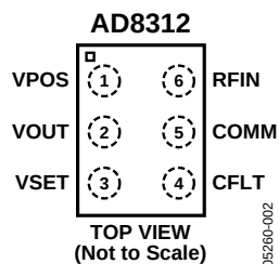
Figure 2. Pin Configuration
