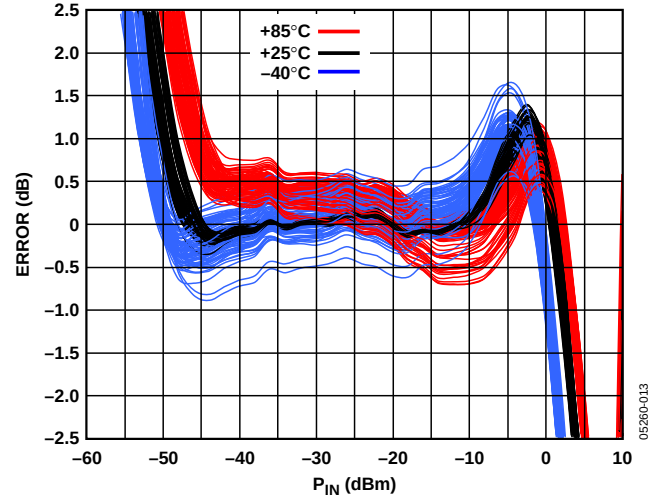
Figure 13. Distribution of Error at -40^{\circ}\text{C} , +25^{\circ}\text{C} , and +85^{\circ}\text{C} After Ambient Normalization vs. Input Amplitude at 2.2 GHz for 80 Devices
