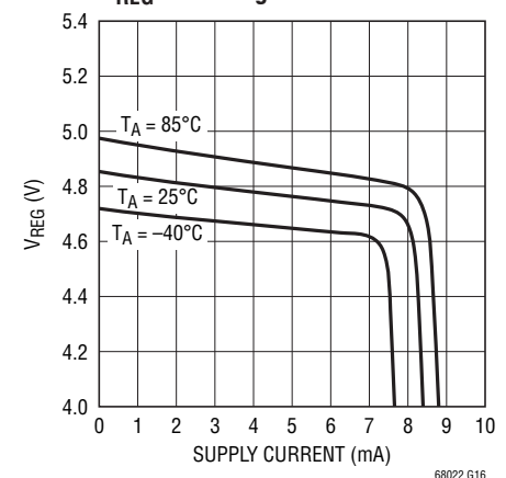
V_{\text{REG}} Load Regulation
