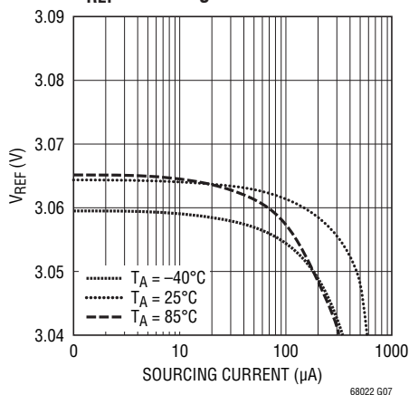
V_{\text{REF}} Load Regulation
