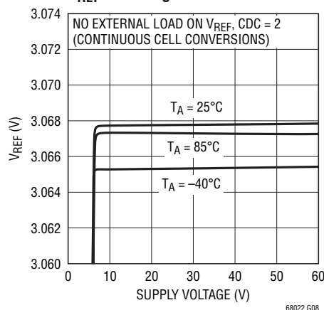
V_{\text{REF}} Line Regulation
