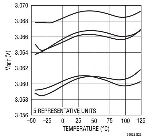
V_{\text{REF}} Output Voltage vs Temperature
