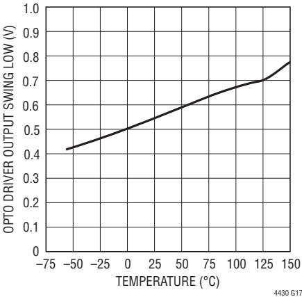
Opto Driver Output Swing Low vs Temperature
