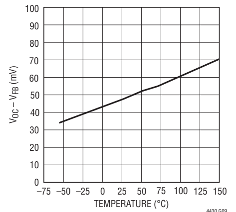
OC Amplifier Offset Voltage vs Temperature
