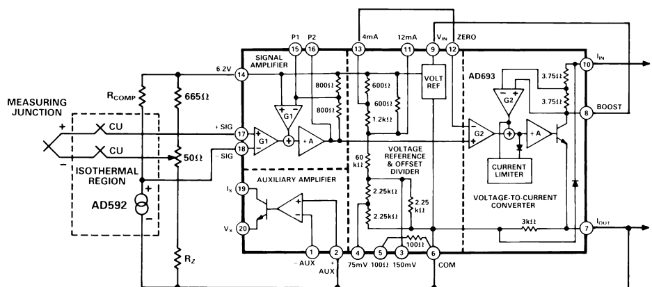
Figure 19. Thermocouple Inputs with Cold Junction Compensation
