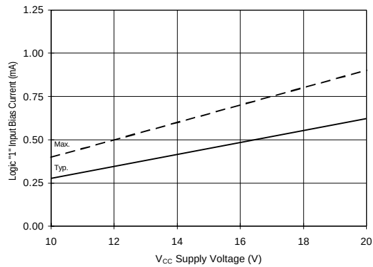
Figure 29A. Logic "1" Input Current vs. Voltage
