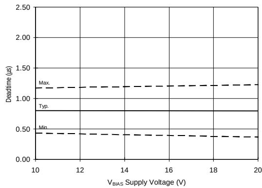
Figure 18D. Deadtime vs. Voltage (IR2132)
