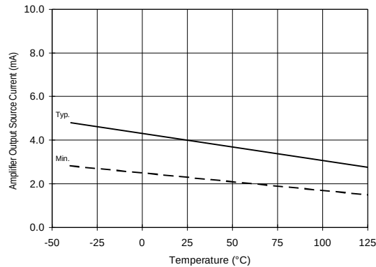
Figure 46A. Amplifier Output Source Current vs. Temperature
