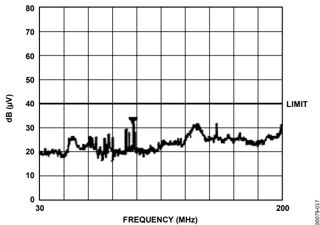
Figure 22. Radiated Emissions
