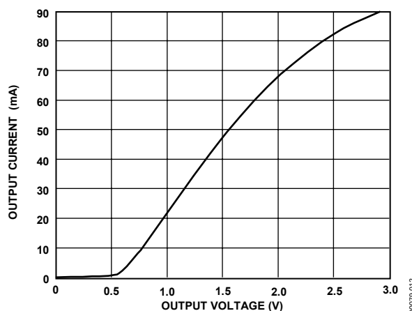
Figure 17. Output Current vs. Driver Output Low Voltage
