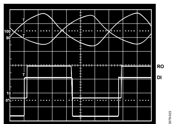
Figure 20. Driving 4000 Ft. of Cable
