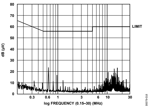
Figure 23. Conducted Emissions
