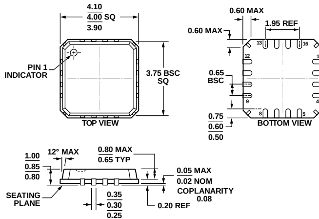
Figure 68. 16-Lead Lead Frame Chip Scale Package [LFCSP_VQ] 4 mm × 4 mm Body, Very Thin Quad, with Hidden Paddle (CP-16-19) Dimensions are shown in millimeters
