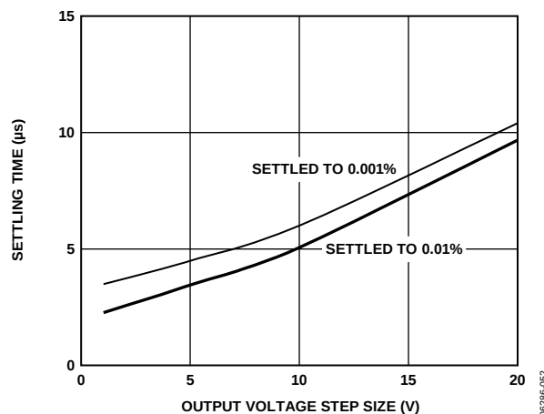
Figure 50. Settling Time vs. Output Voltage Step Size, ( G = 1 ) \pm 15\text{ V} , V_{REF} = 0\text{ V}
