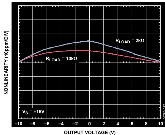
Figure 20. Gain Nonlinearity, G = 1
