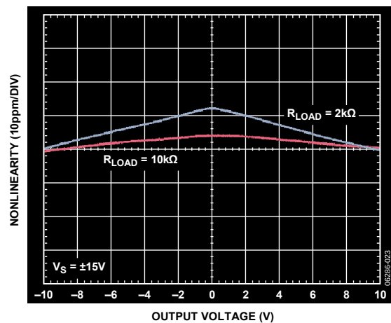
Figure 21. Gain Nonlinearity, G = 10
