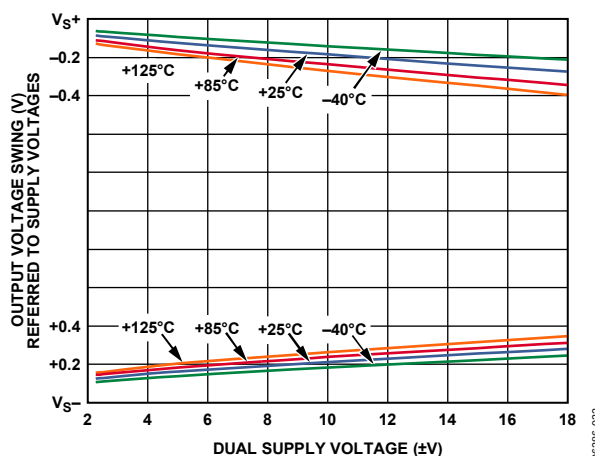
Figure 30. Output Voltage Swing vs. Dual Supply Voltage, R_{LOAD} = 10\text{ k}\Omega , G = 10 , V_{REF} = 0\text{ V}
