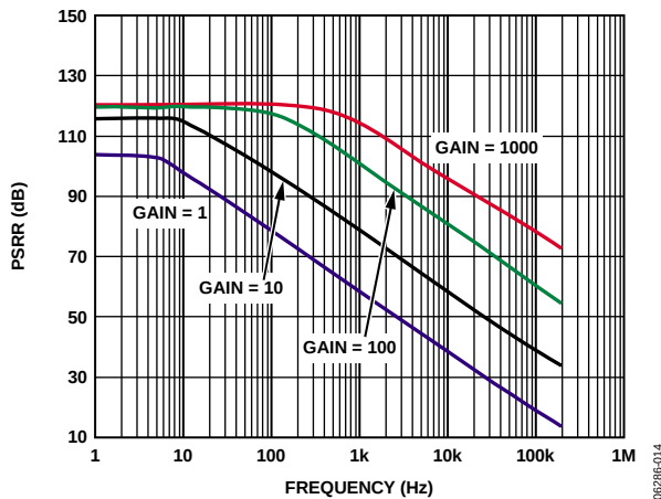
Figure 12. Negative PSRR vs. Frequency, RTI
