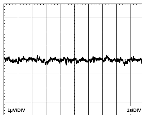
Figure 8. 0.1 Hz to 10 Hz RTI Voltage Noise ( G = 1 )
