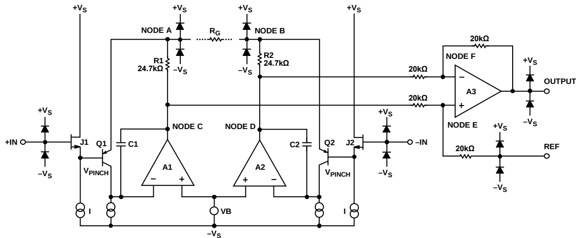
Figure 55. Simplified Schematic
