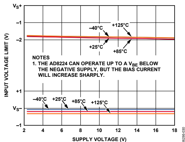
Figure 28. Input Voltage Limit vs. Supply Voltage, G = 1 , V_{REF} = 0\text{ V}
