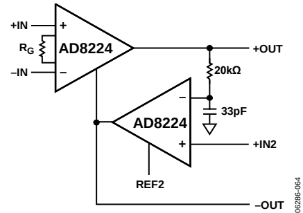
Figure 63. Differential Circuit Schematic
