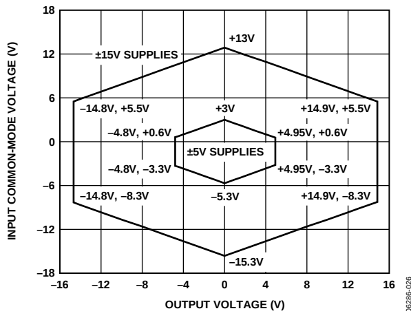
Figure 24. Input Common-Mode Voltage Range vs. Output Voltage, G = 1 , V_{REF} = 0V
