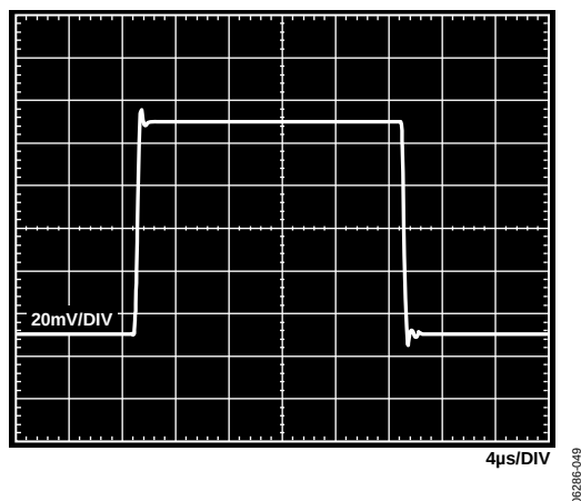
Figure 47. Small Signal Pulse Response, G = 10 , R_{LOAD} = 2\text{ k}\Omega , C_{LOAD} = 100\text{ pF} , V_S = 5\text{ V} , V_{REF} = 2.5\text{ V}
