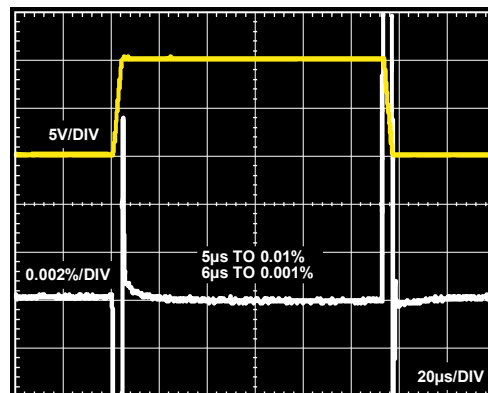
Figure 38. Large Signal Pulse Response and Settle Time, G = 1 , R_{LOAD} = 10\text{ k}\Omega , V_S = \pm 15\text{ V} , V_{REF} = 0\text{ V}
