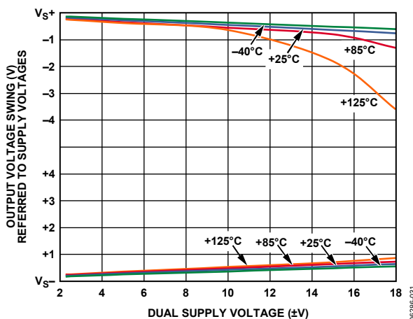
Figure 29. Output Voltage Swing vs. Dual Supply Voltage, R_{LOAD} = 2\text{ k}\Omega , G = 10 , V_{REF} = 0\text{ V}
