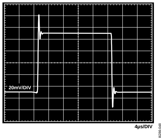
Figure 46. Small Signal Pulse Response, G = 1 , R_{LOAD} = 2\text{ k}\Omega , C_{LOAD} = 100\text{ pF} , V_S = 5\text{ V} , V_{REF} = 2.5\text{ V}
