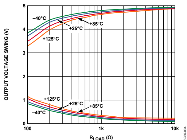
Figure 32. Output Voltage Swing vs. Load Resistance, V_S = 5\text{ V} , V_{REF} = 2.5\text{ V}
