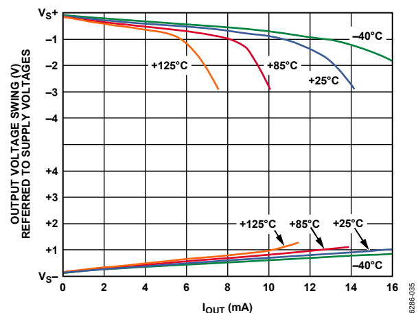
Figure 33. Output Voltage Swing vs. Output Current, V_S = \pm 15\text{ V} , V_{REF} = 0\text{ V}
