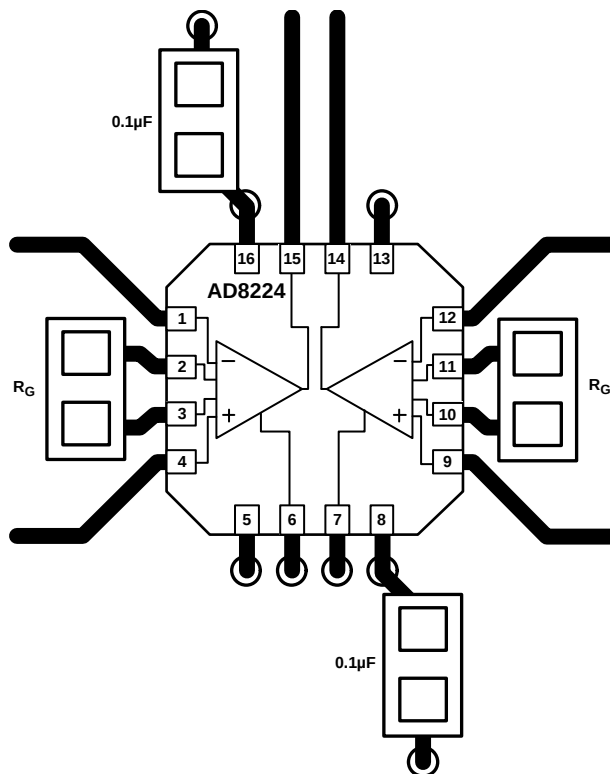
Figure 58. Example Layout
