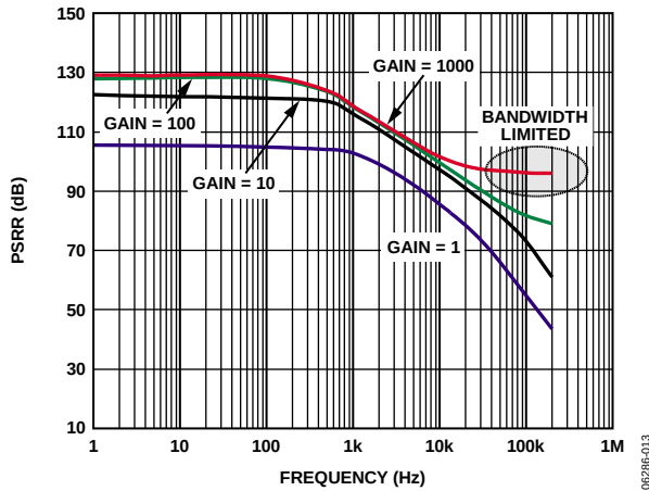
Figure 11. Positive PSRR vs. Frequency, RTI
