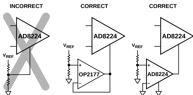
Figure 56. Driving the Reference Pin
