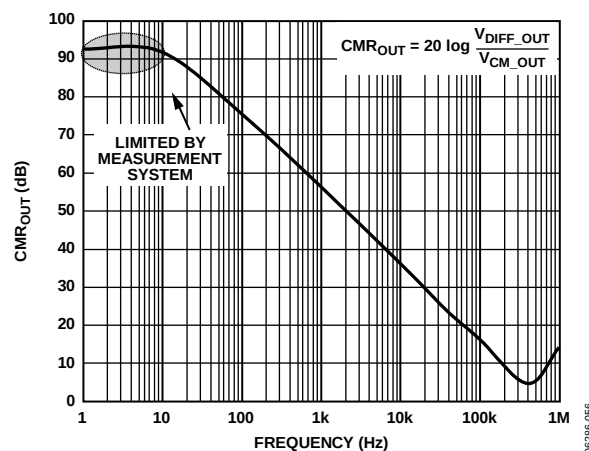
Figure 54. Differential Output Configuration: Common-Mode Output ( CMROUT ) vs. Frequency
