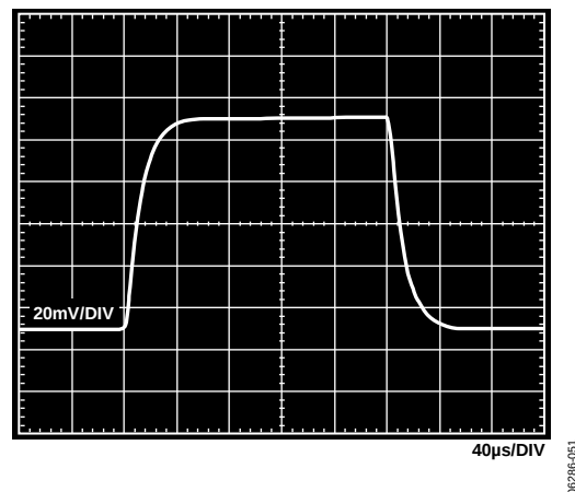
Figure 49. Small Signal Pulse Response, G = 1000 , R_{LOAD} = 2\text{ k}\Omega , C_{LOAD} = 100\text{ pF} , V_S = 5\text{ V} , V_{REF} = 2.5\text{ V}
