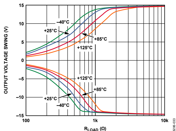
Figure 31. Output Voltage Swing vs. Load Resistance, V_S = \pm 15\text{ V} , V_{REF} = 0\text{ V}
