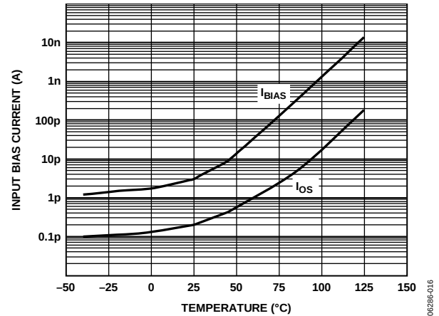
Figure 14. Input Bias Current and Offset Current vs. Temperature, V_S = \pm 15\text{ V} , V_{REF} = 0\text{ V}
