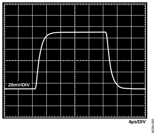
Figure 48. Small Signal Pulse Response, G = 100 , R_{LOAD} = 2\text{ k}\Omega , C_{LOAD} = 100\text{ pF} , V_S = 5\text{ V} , V_{REF} = 2.5\text{ V}
