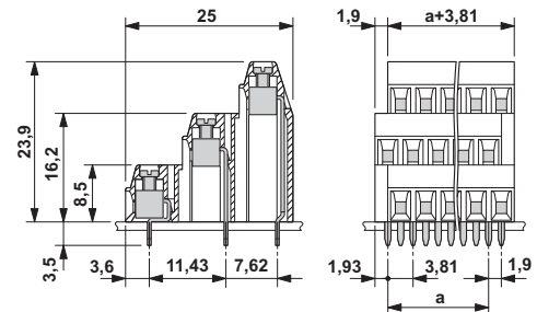
Dimensioned drawing
