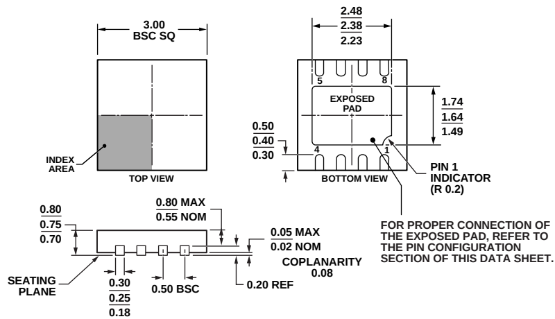
Figure 58. 8-Lead Lead Frame Chip Scale Package [LFCSF_WD] 3 mm x 3 mm Body, Very Very Thin, Dual Lead (CP-8-5)
